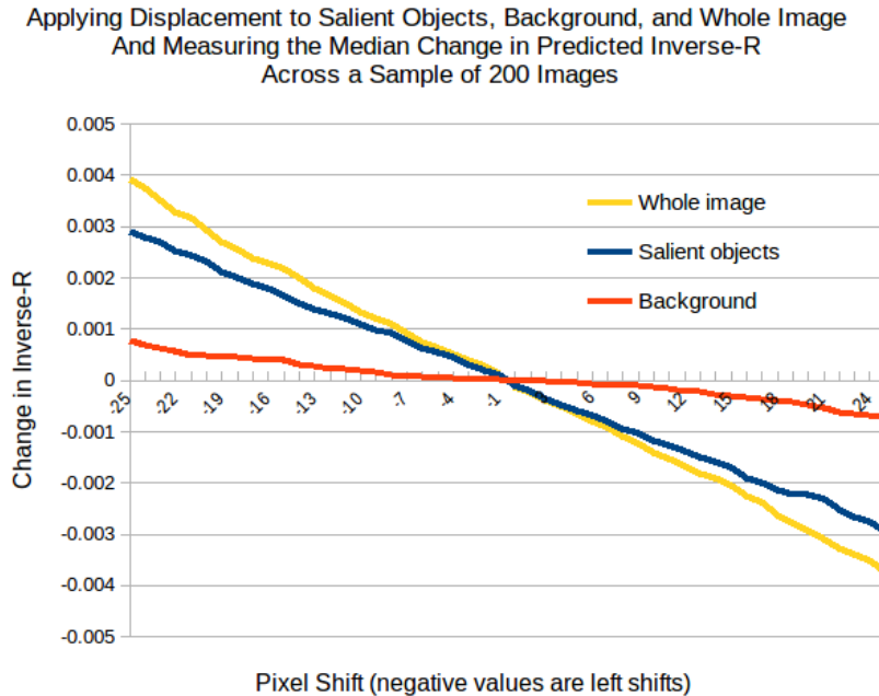
Figure 8: Plots of PilotNet steering output as a function of pixel shift in the input image.
